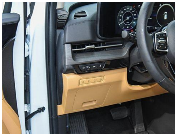
(Optional) Find an appropriate position at the driver's area, drill a \phi 21\text{mm} hole and install the added front switch.
