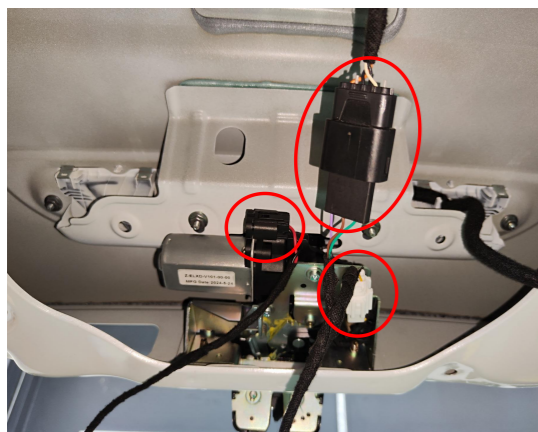
12. Connect the plugs of the lock signal harness to the plugs of the power latch.
