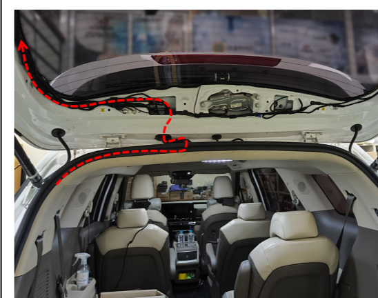
15. Thread the power harness to the tailgate.
