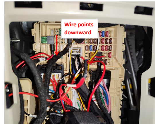
21. Plug the fuse tap into the fuse box and pay attention to the direction.
