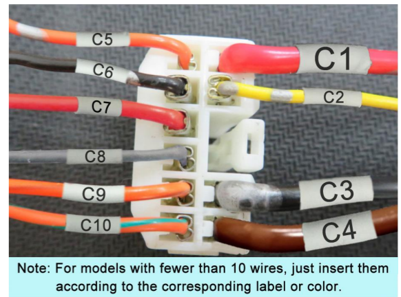
16. Insert the power harness terminals into the connector according to the diagram. Note: For models with fewer than 10 wires, just insert them according to the corresponding label or color.
