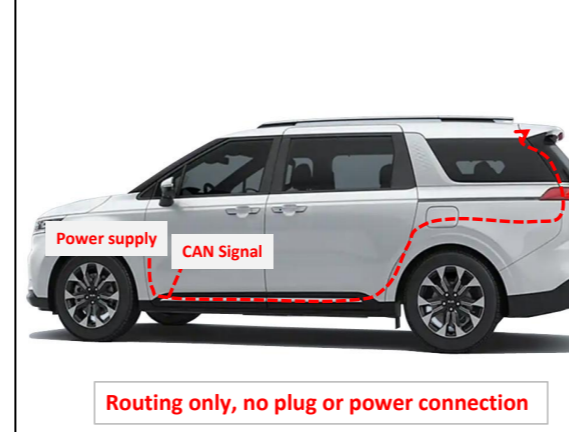
14. Route the power harness (if you need to install the added front switch, route the switch wiring harness in the same way).
