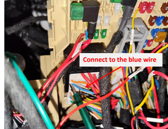
18-1. If you choose not to connect the CAN plugs, connect the orange wire of power harness to the indicated blue
