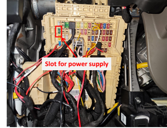
19. The fuse slot for power supply is as indicated.
