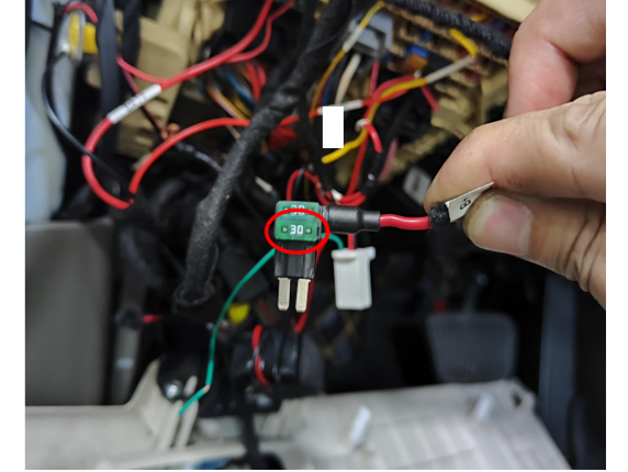
20. Move the fuse from the fuse box to the fuse tap.
