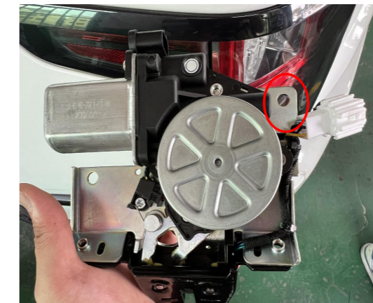
10. Remove the white plug from the indicated position.
