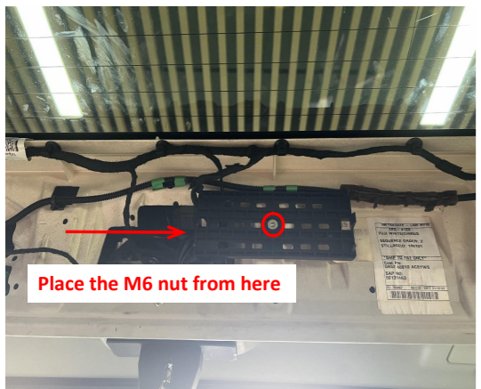
22. Place the M6 nut on the ECU bracket from the indicated direction.
