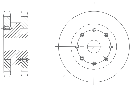
Dimensions for Processing Rivet Holes.
