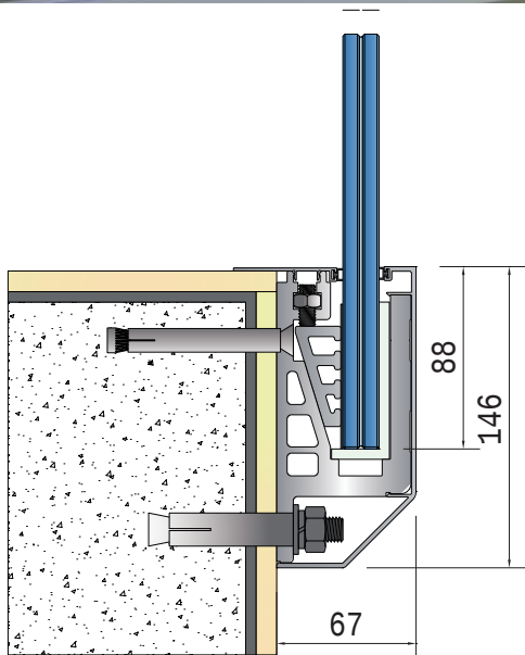
安装方式 Linear Continuous Profile Installation
