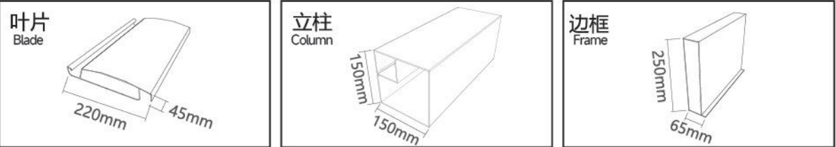
型材截面图 Profile sectional drawing
