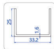
C 左右收边U槽 Right & left U channel
