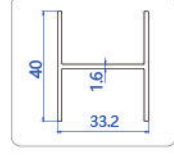
D 中间H槽 Middle H channel
