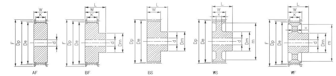
同步带轮基本形状结构图例/Timing belt pulley structure legend
