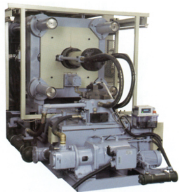
ZLC550 油冷式伺服泵 ZLC-550 Oil Cooled Type Servo Pump
