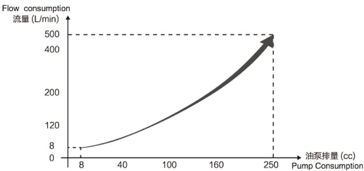
ZLC550 油冷式伺服泵 ZLC-550 Oil Cooled Type Servo Pump
