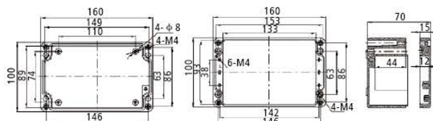
LK161007 product dimensions and mounting hole location
