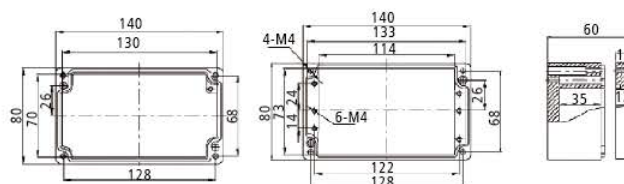
LK140806 product dimensions and mounting hole location
