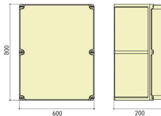
DIMENSION (mm)
