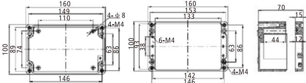
LK161007 product dimensions and mounting hole location
