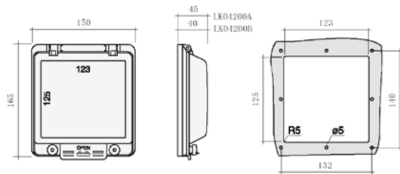
Outline dimension, mounting hole and hole position diagram of LK04-200 window product
