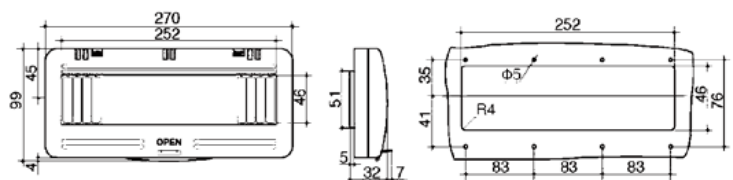
Outline dimension, mounting hole and hole position diagram of LK4-14D window product
