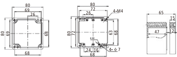
LK080807 product dimensions and mounting hole location
