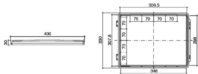
Outline dimension, mounting hole and hole position diagram of LK4-36B window product
