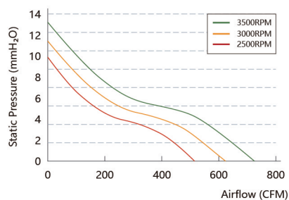
Air Performance
