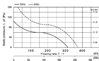
Air Performance
