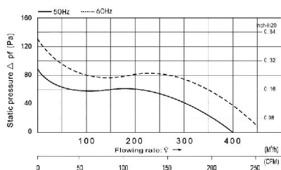
Air Performance
