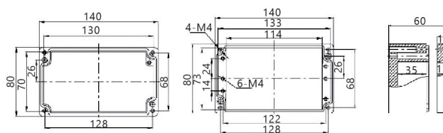
LK140806 product dimensions and mounting hole location
