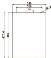
OPENING PROFILE
