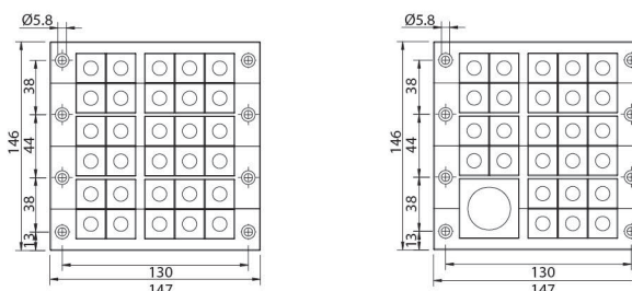
CES 2ET triple row cable entry frame
