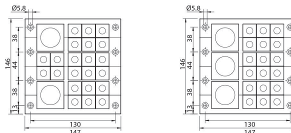
CES 2ET triple row cable entry frame
