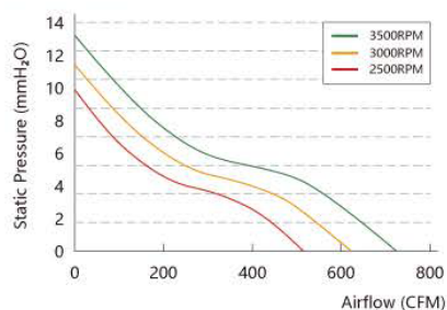
Air Performance
