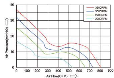
Air Performance
