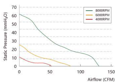
Air Performance
