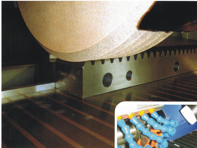
• Germany CNC grinding and milling machine
