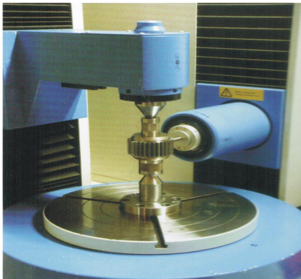
• Testing the pinion
