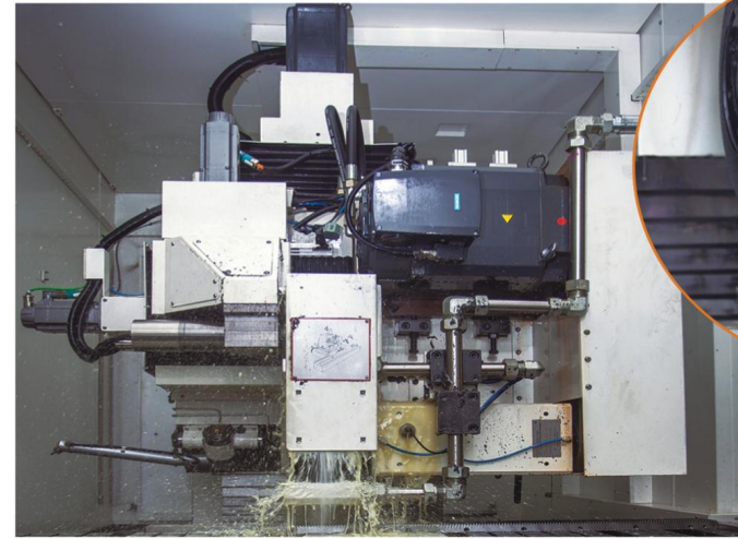
• Grinding the teeth of gear rack
