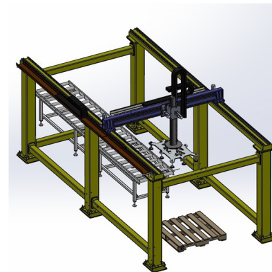
• Heavy truss manipulator / ground rail robot
