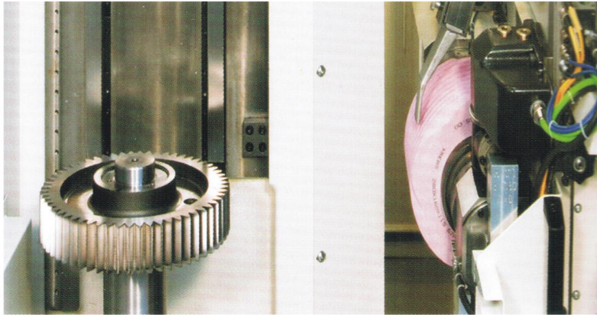
• Grinding the teeth of pinion
