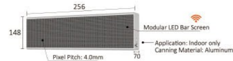
SCREEN LT-LEDPS3 LED MODULAR
