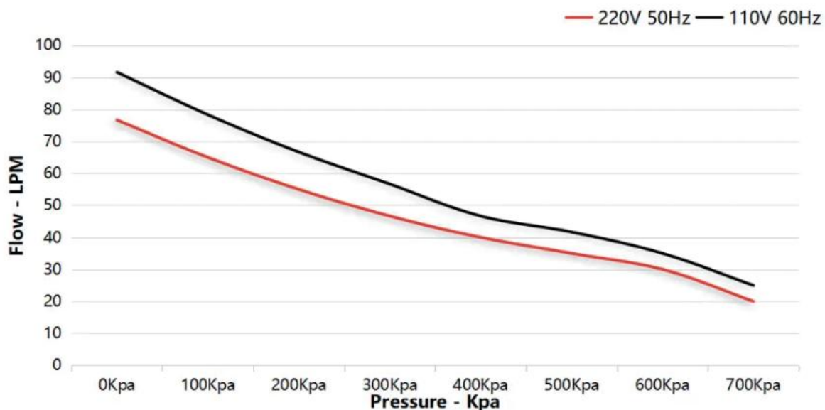
Performance Chart - Flow VS. Pressure
