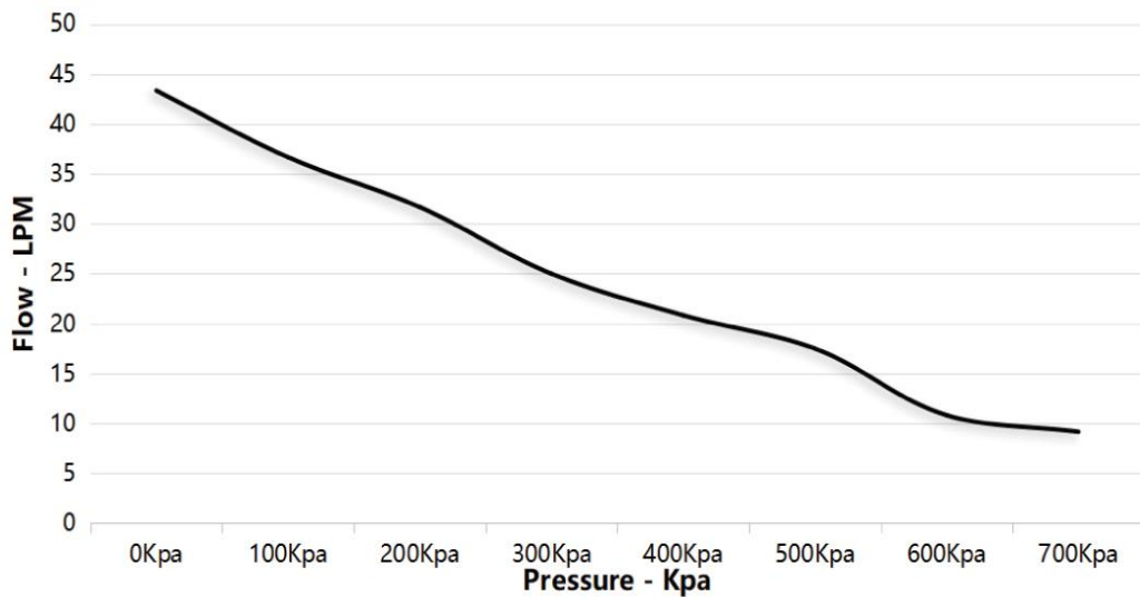
Performance Chart - Flow VS. Pressure
