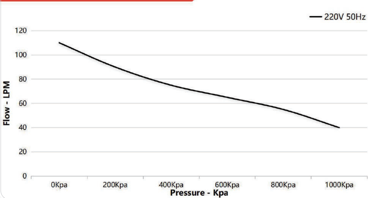
Performance Chart - Flow VS. Pressure
