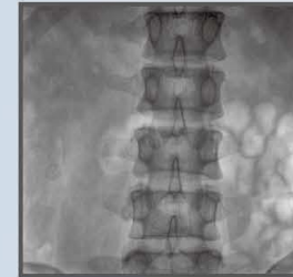
✓ Lumbar fluoroscopy
