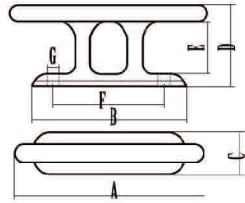
方孔码头缆桩 Dock Bollard
