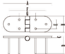
带丝杆合页 Casting Hinge
