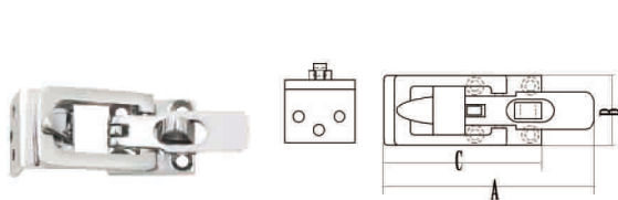
箱包扣 Anti-Rattle Latch Fastener
