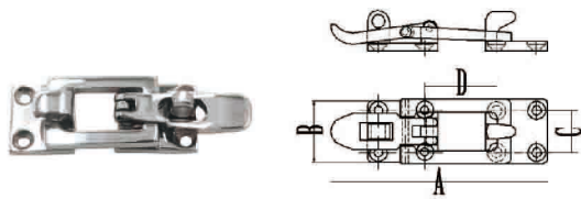
箱包扣 Anti-Rattle Latch Fastener
