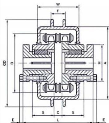
Bushed Type G and H Couplings
