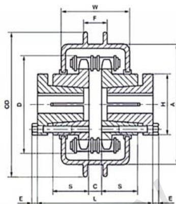
Bushed Type P1, Q1 and R1 Couplings
