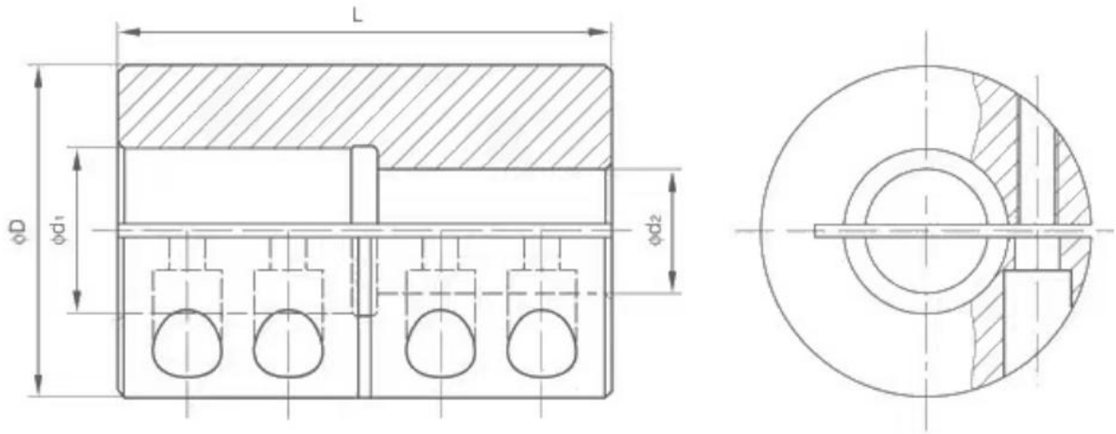
NSPT CC-Coupling 图纸
