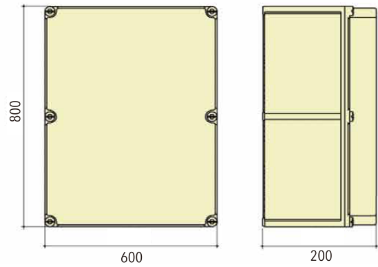
DIMENSION (mm)
