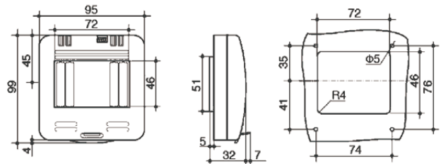
Outline dimension, mounting hole and hole position diagram of LK4-04D window product
