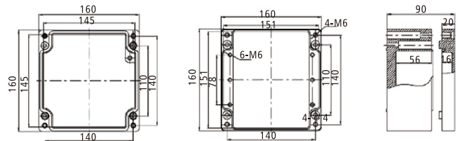
LK161609 product dimensions and mounting hole location
