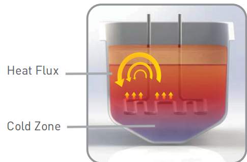
V-shape Oil Tank & Cold Zone
