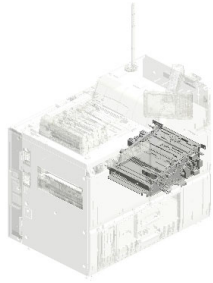
U013 PAPER FEED(MAIN)
