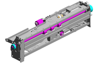
382.D2706628 PAPER FEED UNIT :PAPER BANK:ASS' Y
