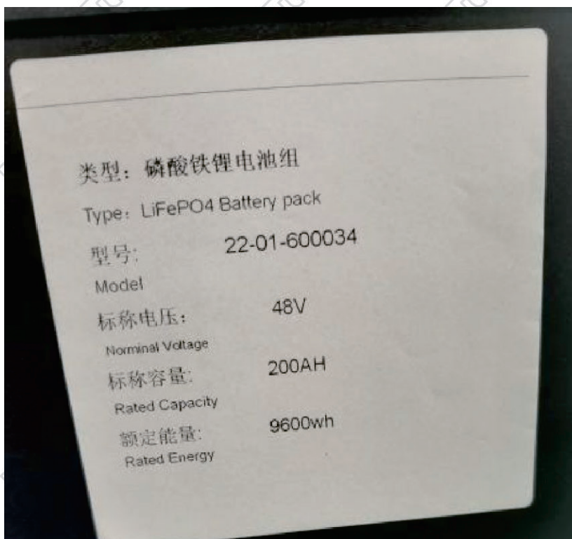
Figure 4 Battery Label (电池标签)
