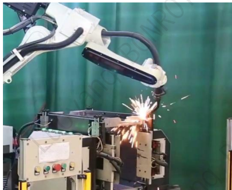
➤ Robot welding
