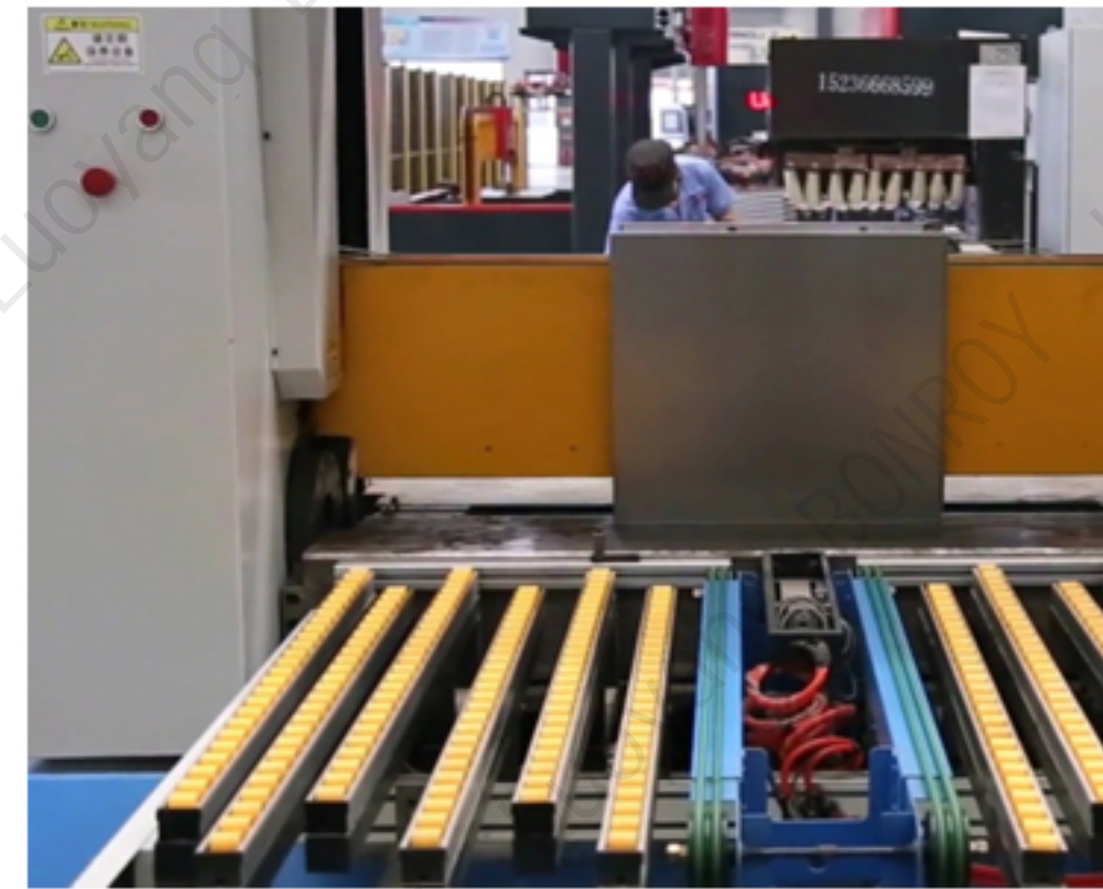
➤ CNC bending
