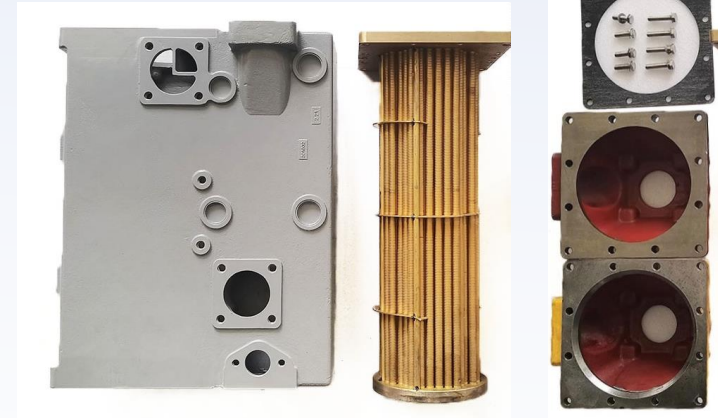
F.w cooler case + element + cover
