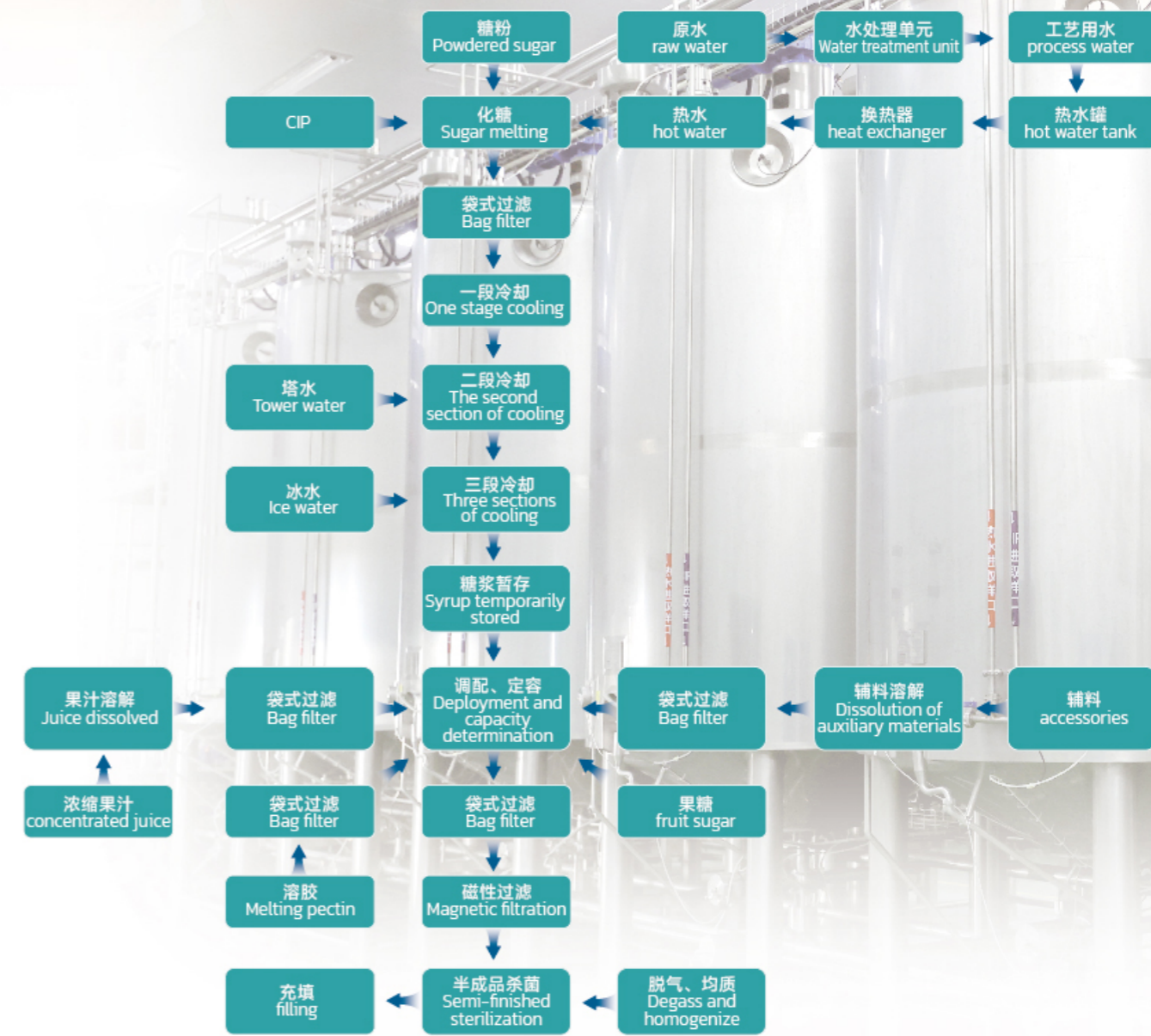
Pre-processing production line process flow chart
