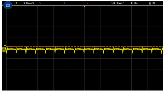
Figure 7, Output ripple & noise (Iout = 30A)
