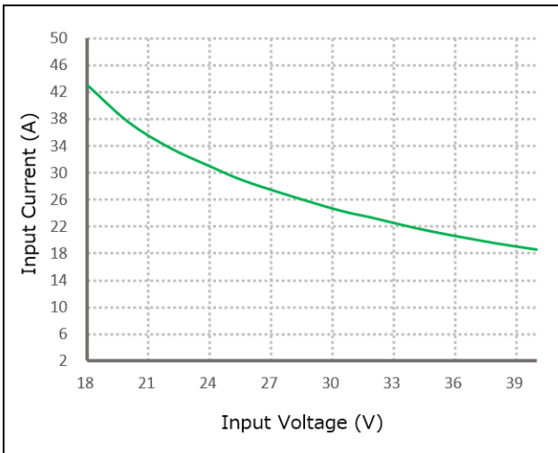
Figure 3, Input V-I, Iout=30A
