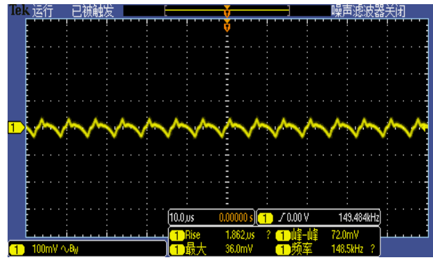
Figure 7, Output ripple & noise (Iout = 10A)
