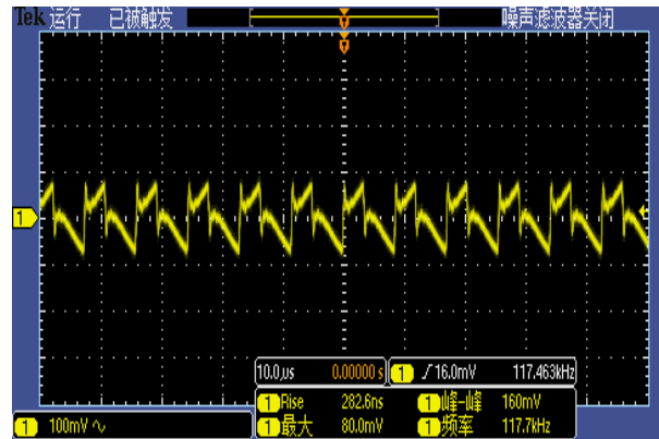
Figure 7, Output ripple & noise (Iout = 10A)
