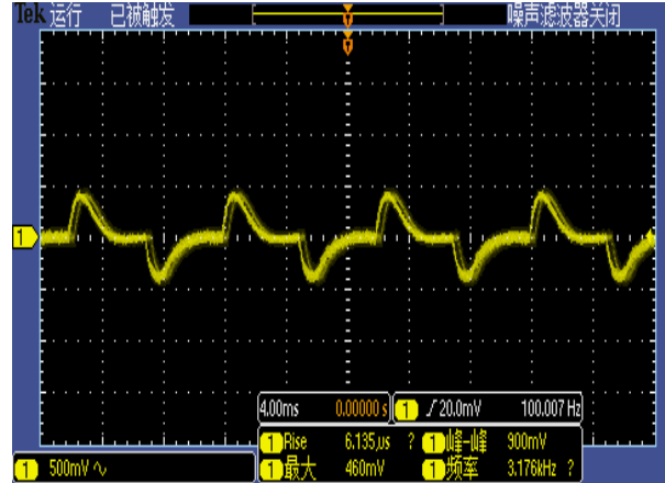
Figure 5, 50% - 75% load dynamic
