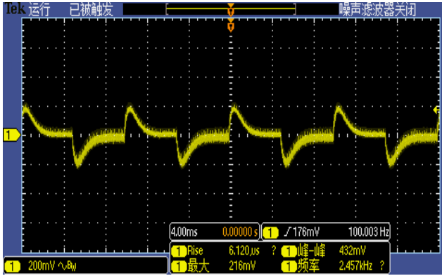
Figure 4, 25% - 50% load dynamic
