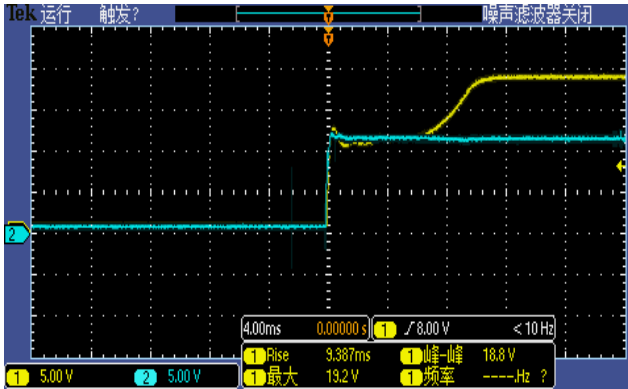
Figure 6, Output voltage established (Iout = 10A)
