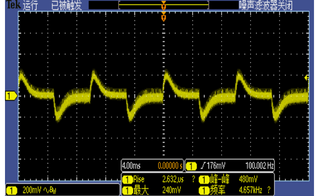
Figure 5, 50% - 75% load dynamic
