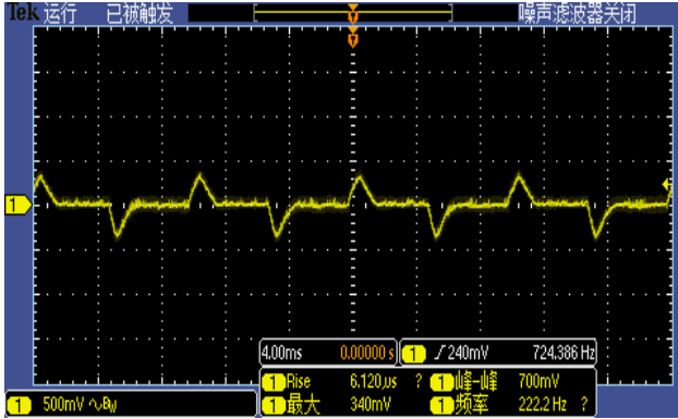
Figure 4, 25% - 50% load dynamic
