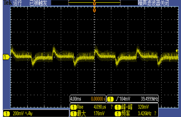
Figure 5, 50% - 75% load dynamic
