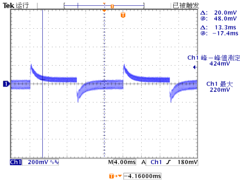
Figure 4, 25% - 50% load dynamic
