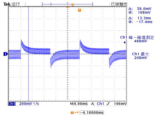
Figure 5, 50% - 75% load dynamic
