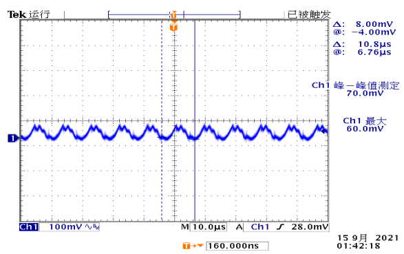
Figure 7, Output ripple & noise (Iout = 30A)
