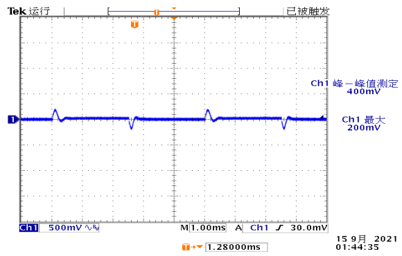
Figure 5, 50% - 75% load dynamic
