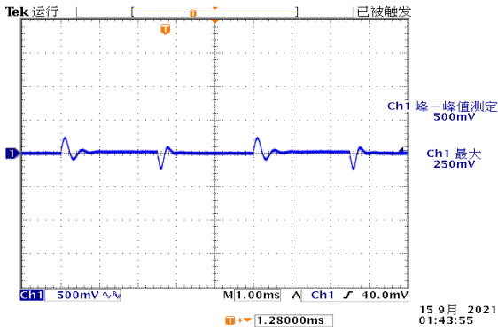
Figure 4, 25% - 50% load dynamic
