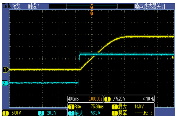
Figure 8, Boot delay time (Iout = 40A)
