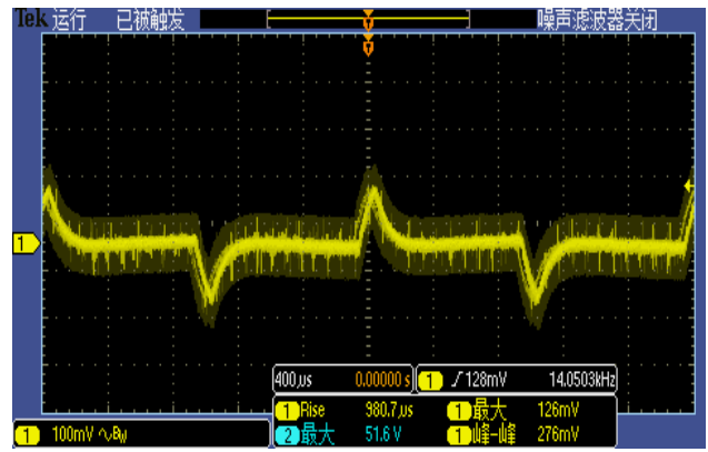
Figure 5, 50% - 75% load dynamic
