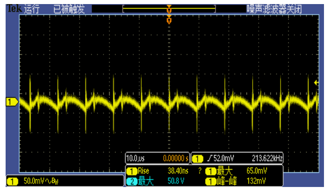
Figure 7, Output ripple & noise (Iout = 40A)
