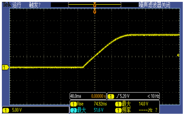
Figure 6, Output voltage established (Iout = 40A)
