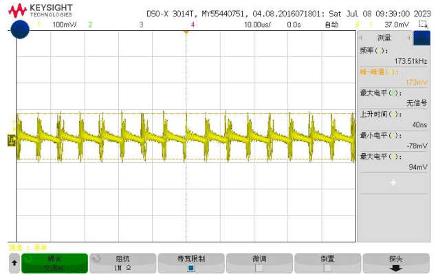
Figure 7, Output ripple & noise (Iout = 32A)
