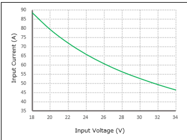
Figure 3, Input V-I, Iout=32A
