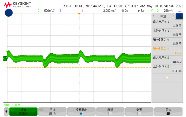
Figure 5, 50% - 75% load dynamic
