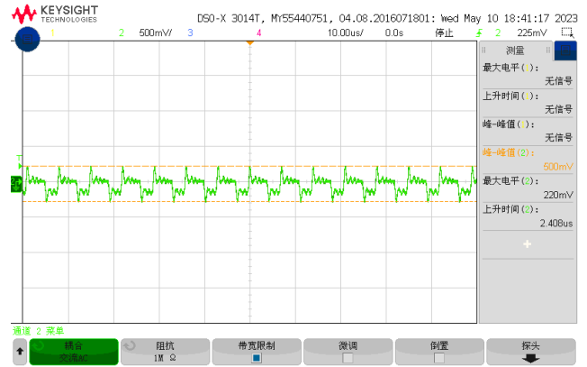
Figure 7, Output ripple & noise (Iout = 5A)
