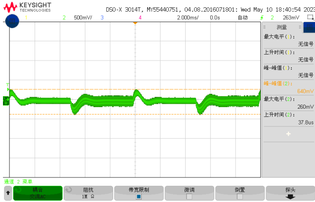
Figure 4, 25% - 50% load dynamic
