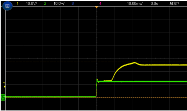
Figure 6, Output voltage established (Iout = 3A)
