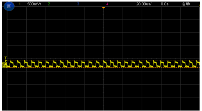
Figure 7, Output ripple & noise (Iout = 3A)
