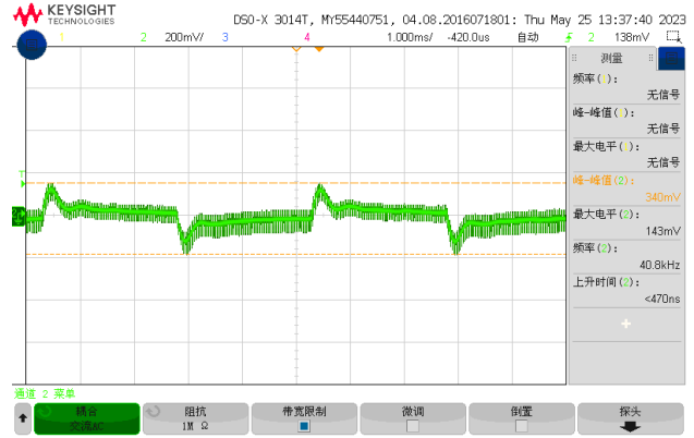
Figure 5, 50% - 75% load dynamic
