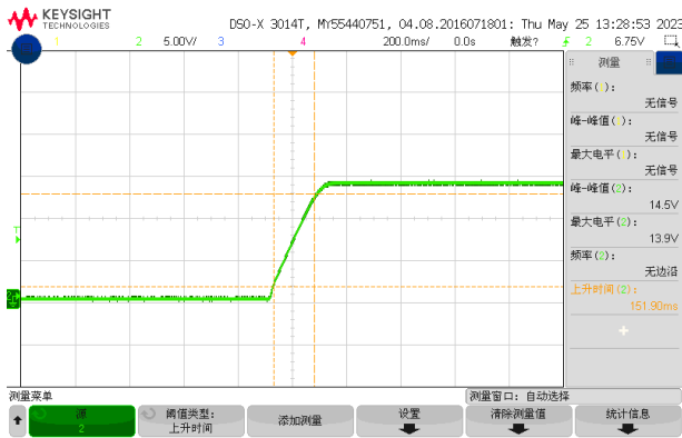
Figure 6, Output voltage established (Iout = 25A)
