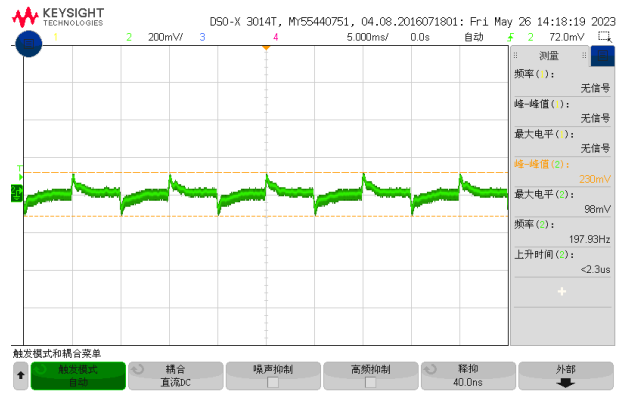
Figure 5, 50% - 75% load dynamic
