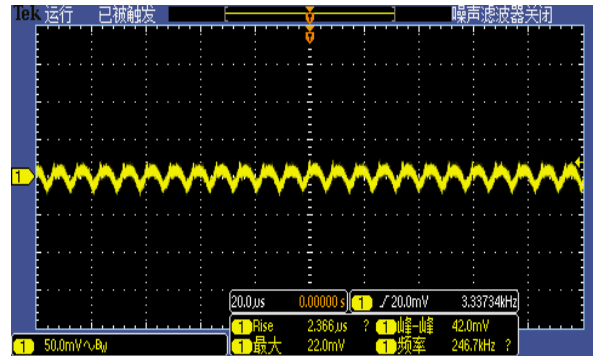
Figure 7, Output ripple & noise (Iout = 20A)
