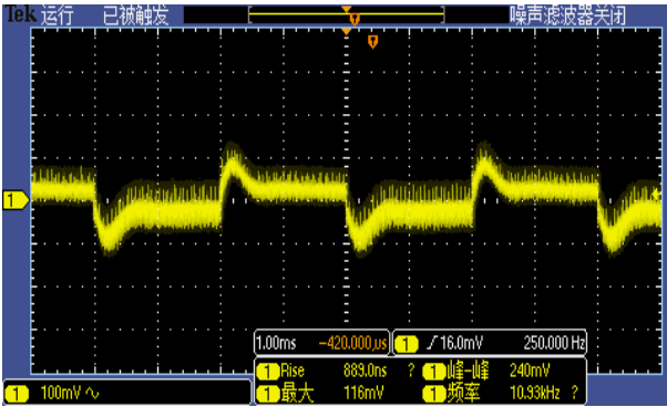
Figure 4, 25% - 50% load dynamic
