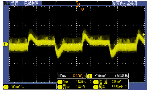
Figure 5, 50% - 75% load dynamic
