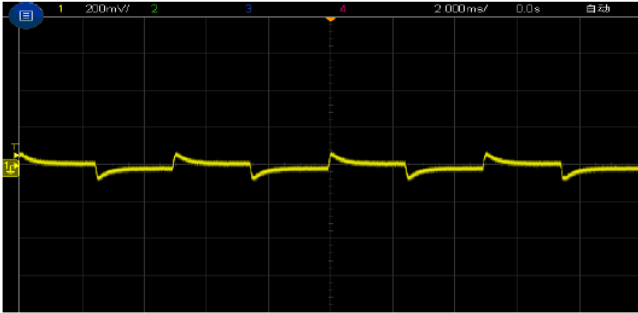
Figure 4, 25% - 50% load dynamic
